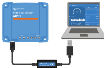
VictronConnect App connection via USB using a VE.Direct USB interface
